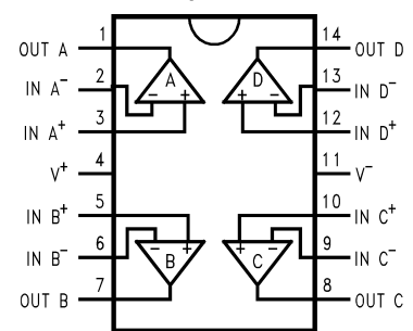
D and PW Package 14-Pin SOIC, TSSOP Top View
