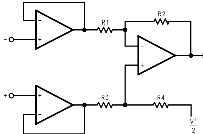
Figure 57. Three-Op-Amp Instrumentation Amplifier
