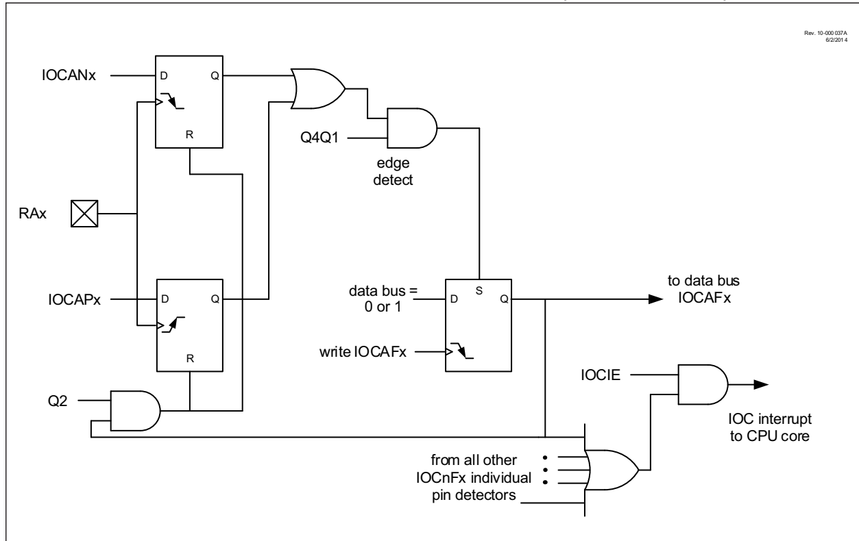
FIGURE 15-1: INTERRUPT-ON-CHANGE BLOCK DIAGRAM (PORTA EXAMPLE)
