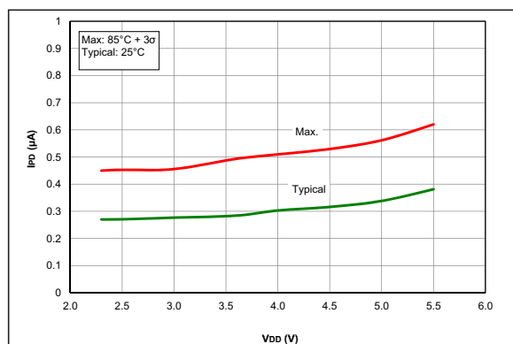
FIGURE 36-25: IPD BASE, 11, PIC16F18325/18345 Only
