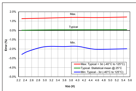
FIGURE 36-27: HFINTOSC Typical Frequency Error, PIC16F18325/18345 Only
