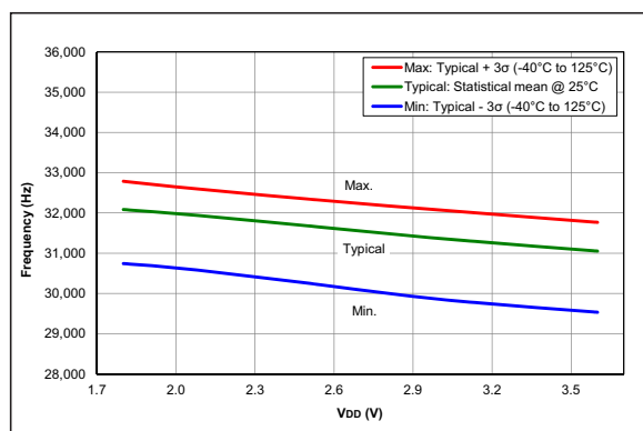
FIGURE 36-29: LFINTOSC Frequency, PIC16LF18325/18345 Only
