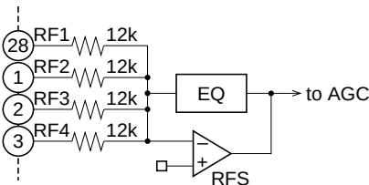
Figure 3 RFS Amplifier
