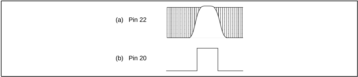
Figure 10 Defect Detection Waveform
