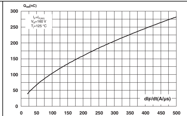
Figure 6. Reverse recovery charges versus dl_F/dt (typical values, per diode)
