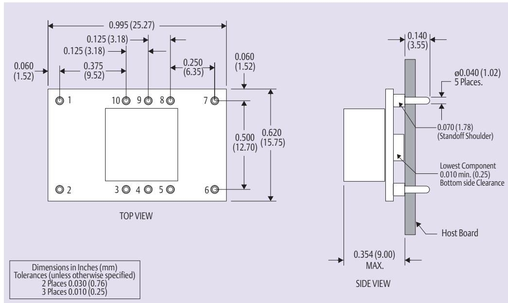
Figure 5 - Plated Through-Hole
