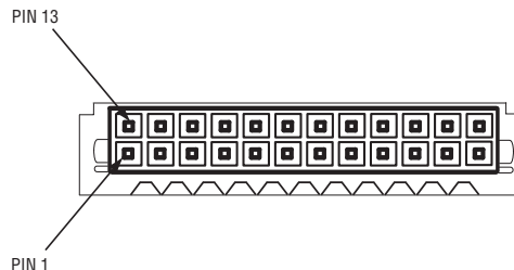
Connector: Molex (15-06-0241)
