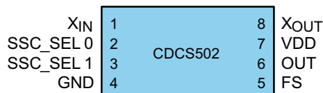
PIN FUNCTIONS
