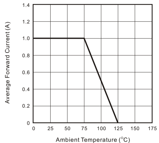
Fig.6 Current Derating Curve
