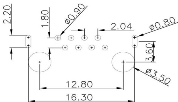
PCB
