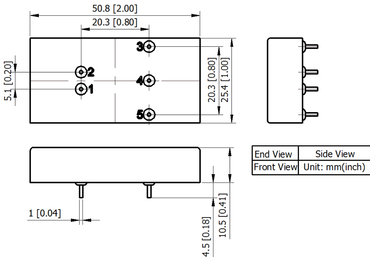
Figure 6. Outline Dimensions
