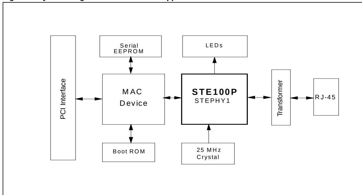
Figure 1. System Diagram of the STE100P Application
