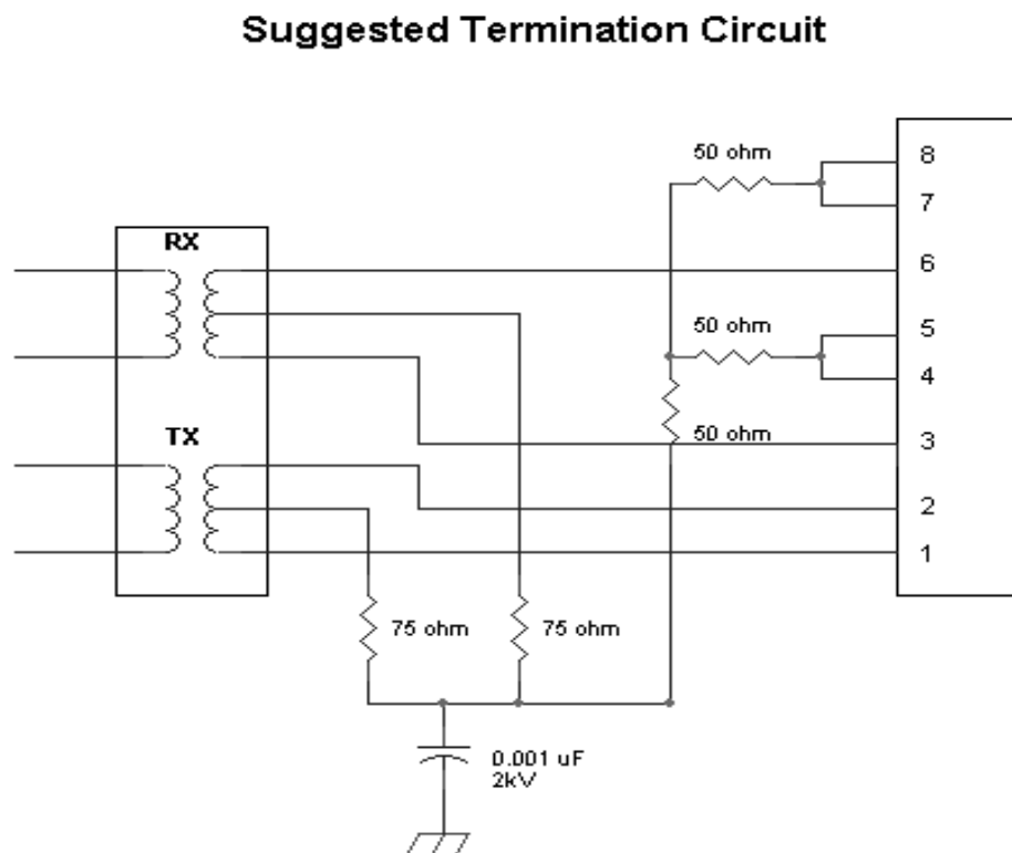
Figure 4. Suggested Termination Circuit
