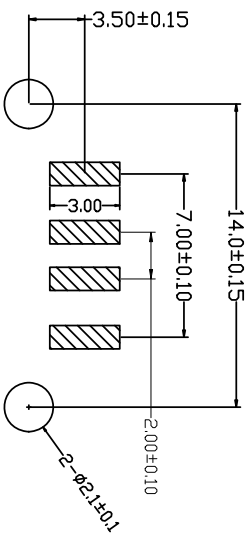
PCB LAYOUT
