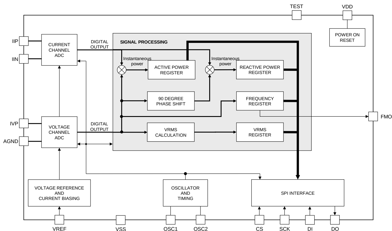
Figure 1: Block diagram
