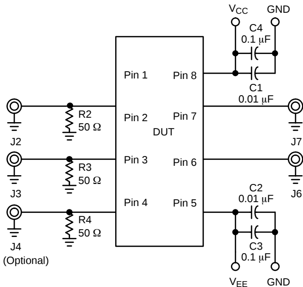
Figure 8. Configuration 5 Schematic
