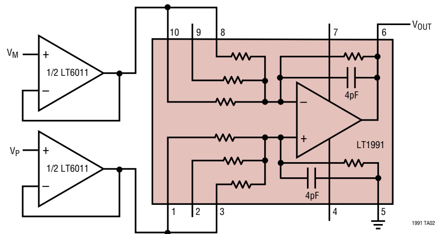
Micropower A_V = 10 Instrumentation Amplifier
