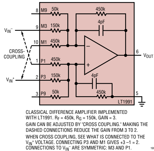
Figure 12. Another Method of Selecting Difference Gain Is "Cross-Coupling." The Additional Method Means the LT1991 Provides All Integer Gains from 1 to 13
