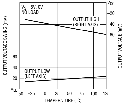
Output Voltage Swing vs Temperature
