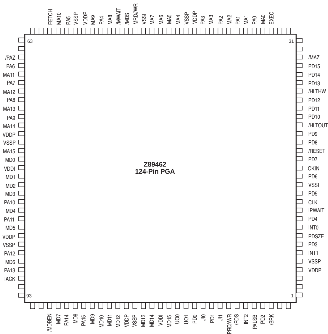
124-Pin PGA Pin Assignments
