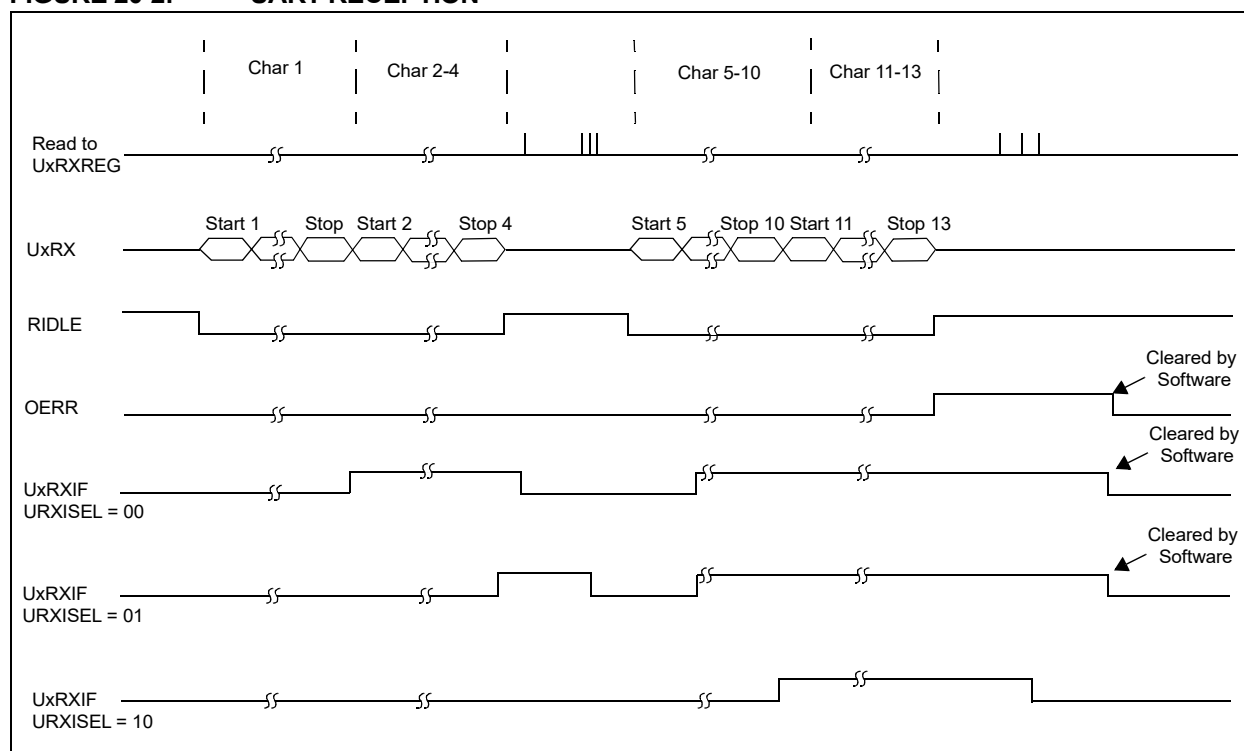
FIGURE 20-2: UART RECEPTION
