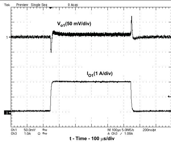
Figure 17. 0-A to 2-A Load Transient Response
