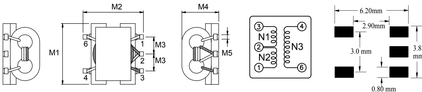
Mechanical dimension
