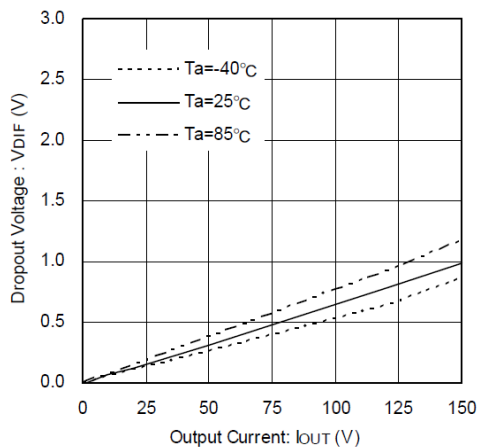
IXD1216B/D C02xx
