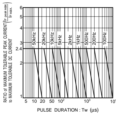
Fig. 26 Maximum tolerable peak current vs. pulse duration
