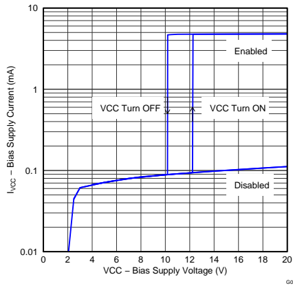
Figure 1. Bias Supply Current vs Bias Supply Voltage
