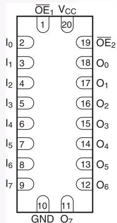
Pad Assignment for DQFN
