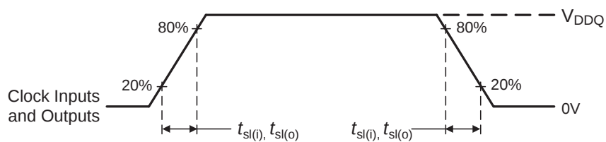
Figure 8. Input and Output Slew Rates
