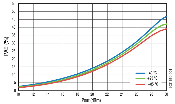
Figure 4. PAE vs. Pout Across Temperature @ 1842.5 MHz, 5 V
