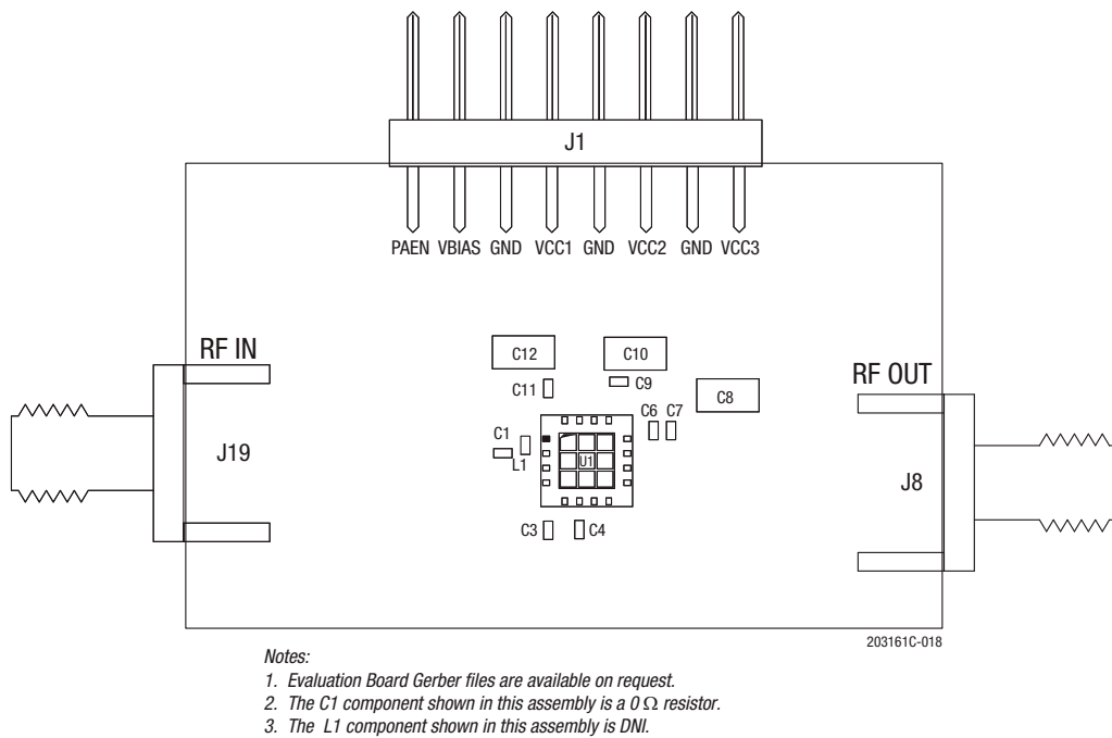
Figure 18. Evaluation Board Assembly Drawing
