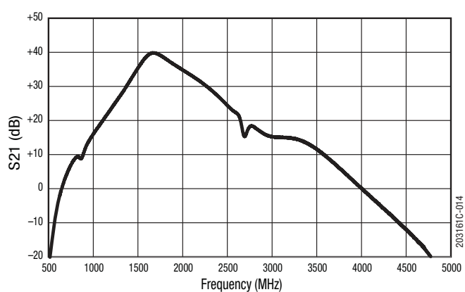
Figure 14. Wide Band Small Signal Gain vs Frequency (PIN = -30 dBm)
