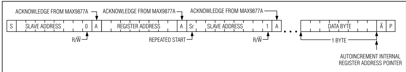
Figure 12. Reading n-Bytes of Indexed Data from the MAX9877A
