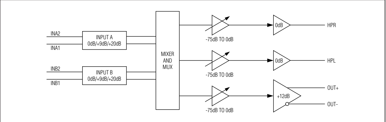
Figure 1. Signal Path
