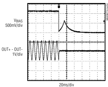
HARDWARE SHUTDOWN RESPONSE
