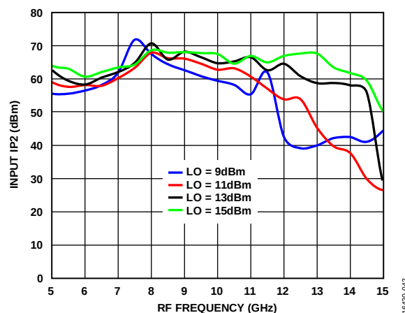
Figure 40. Input IP2 vs. RF Frequency at Various LO Power Levels, T_A = 25^\circ\text{C}
