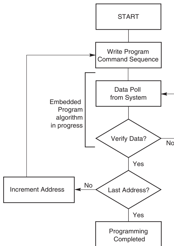
Figure 15.1 Program Operation
