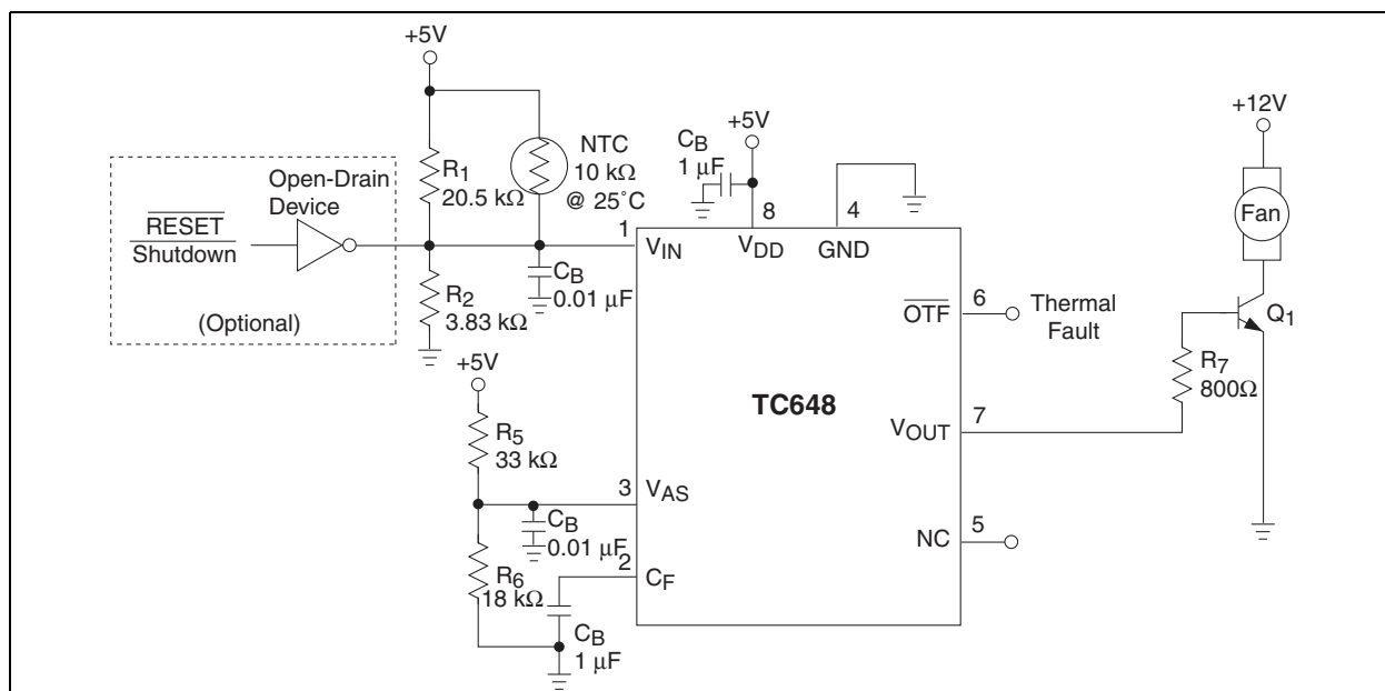
FIGURE 5-8: Design Example.
