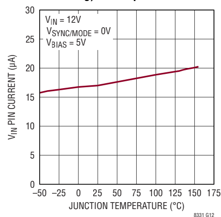
V_{IN} Pin Current (Active Mode, Not Switching) vs Temperature
