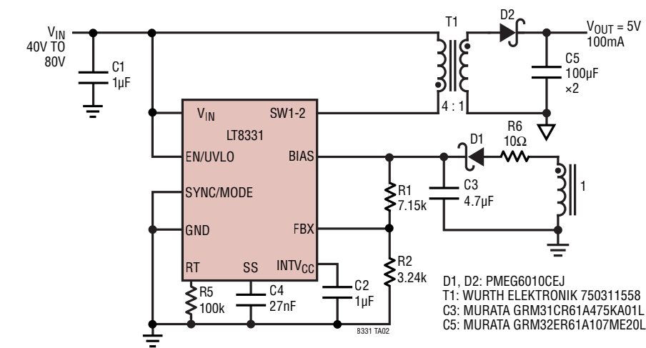
40V to 80V Input, 5V Isolated Output Converter
