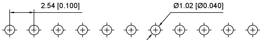
PCB LAYOUT
