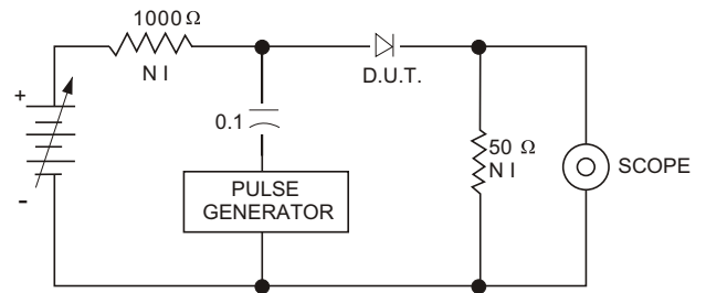
CIRCUIT
