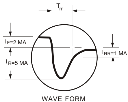
WAVE FORM
