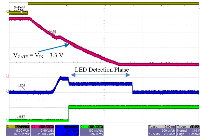
Figure 7: Startup showing EN/PWM, GATE, LED1, and ISET. Note that LED Detection Phase starts as soon as GATE pin is pulled down to 3.3 V below V_{IN} .
