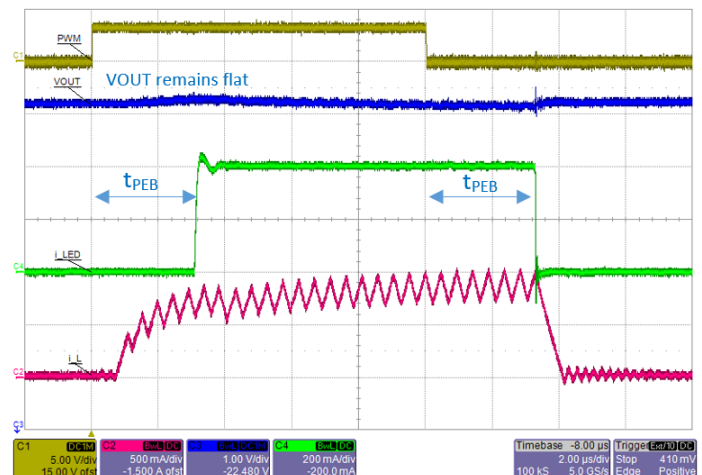
Figure 22: A80602 PWM dimming operation with PEB delay set to 3 \mu s. Note that V_{OUT} ripple is reduced to ~0.2 V.
