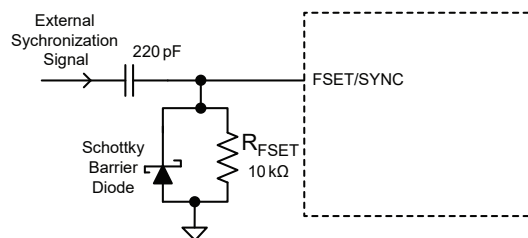
Figure 16: Countermeasure for External Sync Stuck-at-Low Fault
