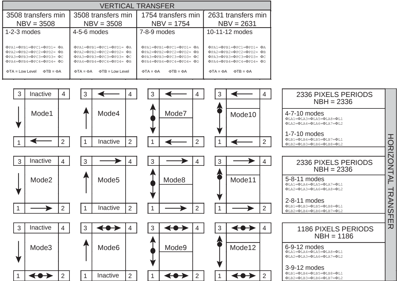
Figure 4. Operating Modes
