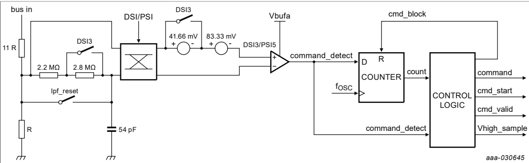
Figure 62. Command receiver physical layer
