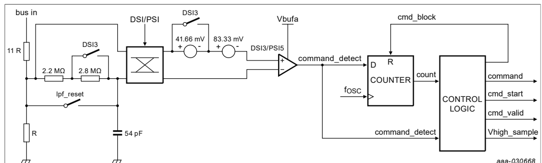
Figure 83. Synchronization pulse detection circuit
