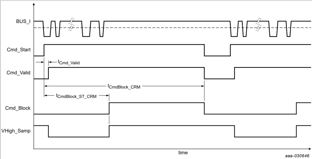
Figure 63. DSI3 command receiver timing diagram: valid command
