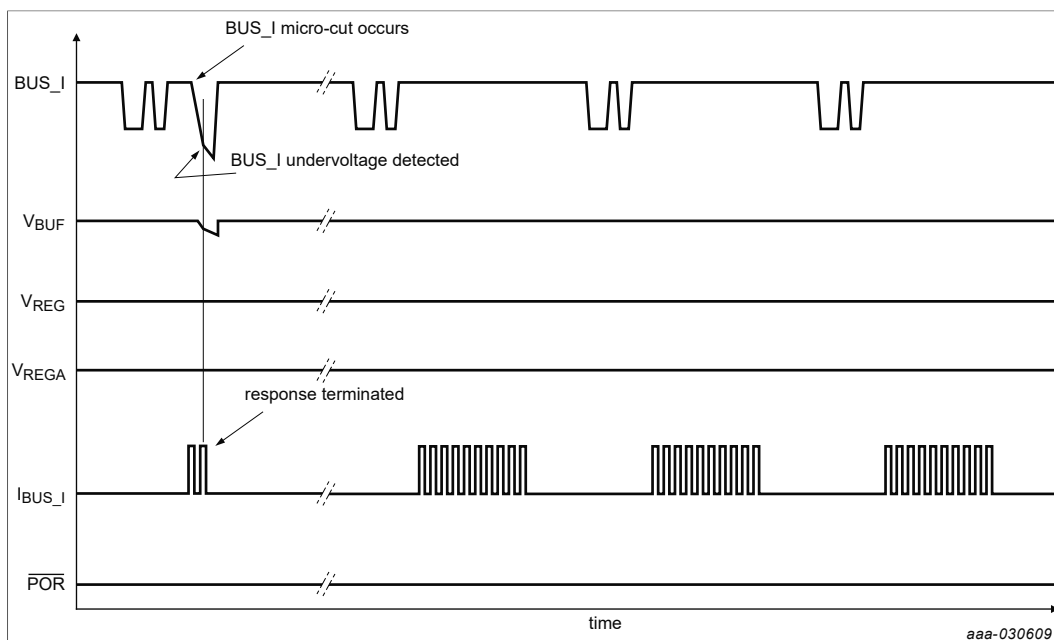
Figure 15. BUS_I micro-cut response (DSI3 or PSI5)
