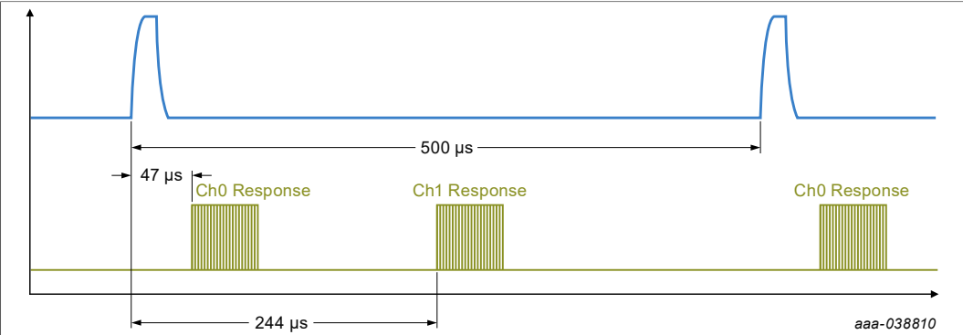
Figure 93. PSI5 default mode transmission
