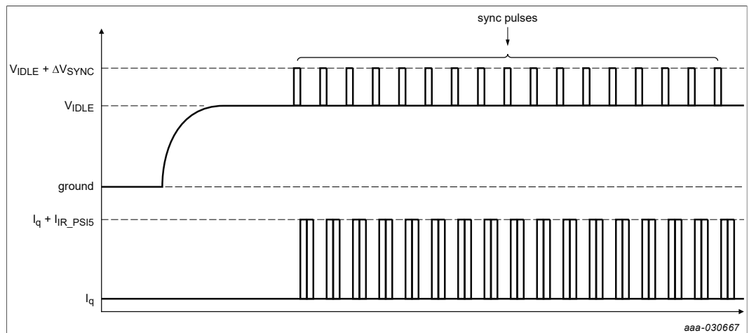
Figure 82. Synchronous communication overview
