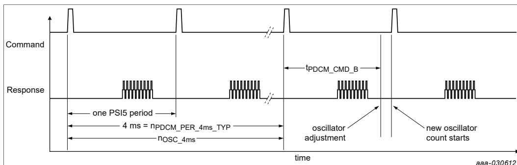
Figure 18. PSI5 oscillator training timing diagram
