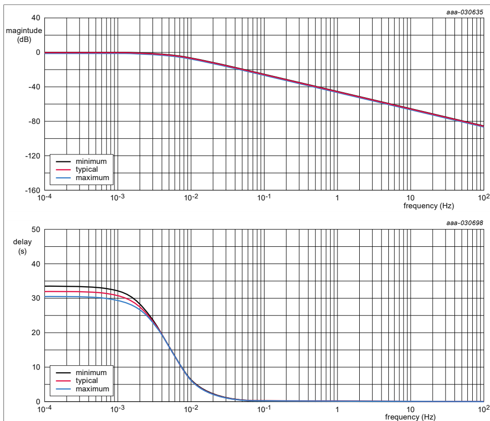
Figure 52. 0.005 Hz offset cancellation low-pass filter characteristics
