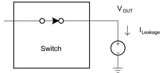
图 10. Switch On Leakage Current
