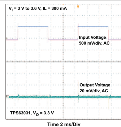
Figure 21. Line Transient Response, TPS63031
