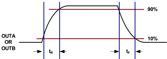
FIGURE 4. RISE/FALL TIMES
