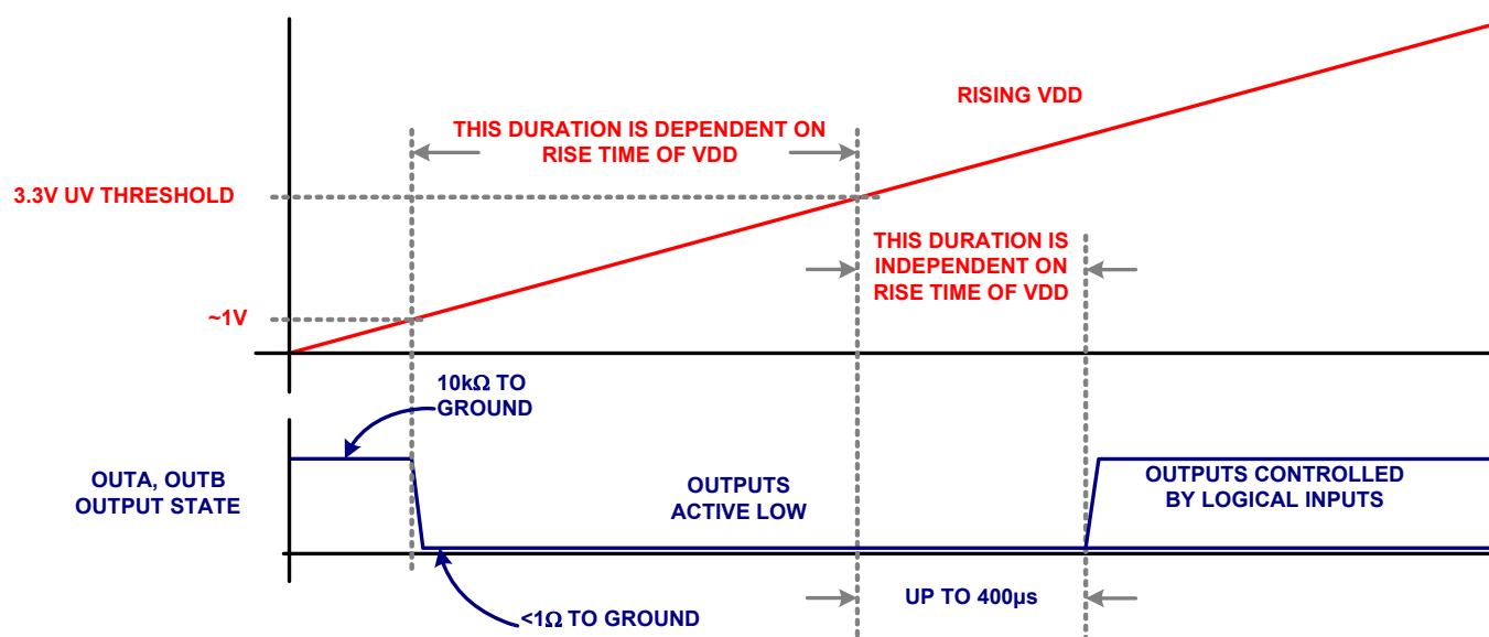
FIGURE 9. START-UP SEQUENCE
