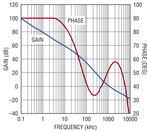
A_{VOL} and Phase vs Frequency
