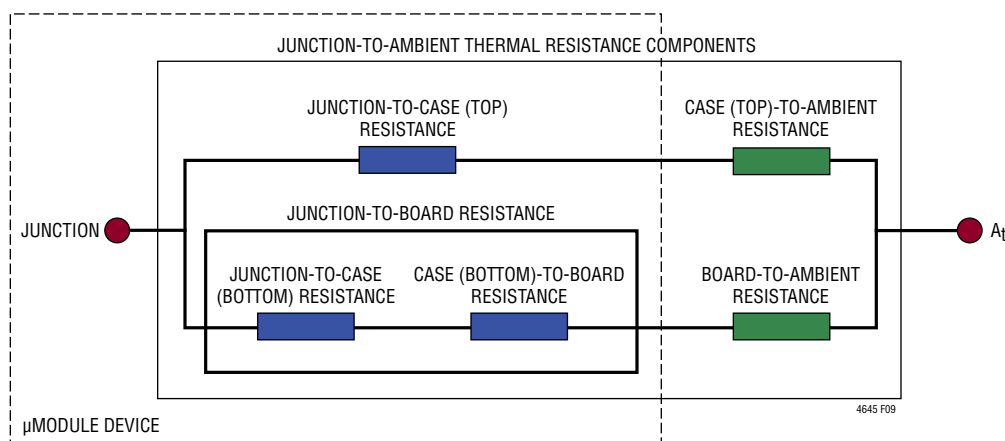
Figure 9. Graphical Representation of JEDEC 51-12 Thermal Coefficients
