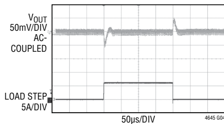
0.9V Output Load Step Transient Response
