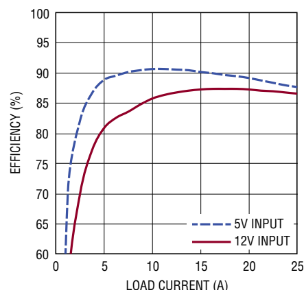
Efficiency vs Output Current at 1V Output
