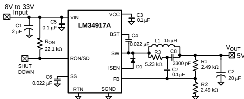
Figure 6. Example Circuit
