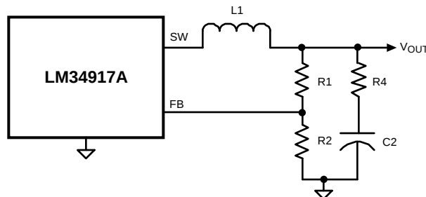
Figure 10. Maximum Ripple Configuration
