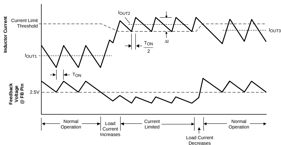
Figure 5. Inductor Current - Normal and Current Limit Operation
