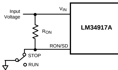
Figure 4. Remote Shutdown
