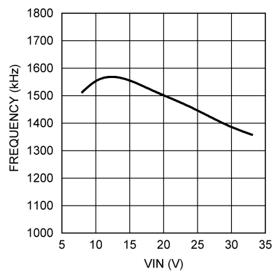
Figure 8. Frequency vs. V_{IN} (Circuit of Figure 4)
