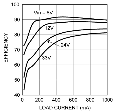
Figure 7. Efficiency vs. Load Current and V_{IN} (Circuit of Figure 4)
