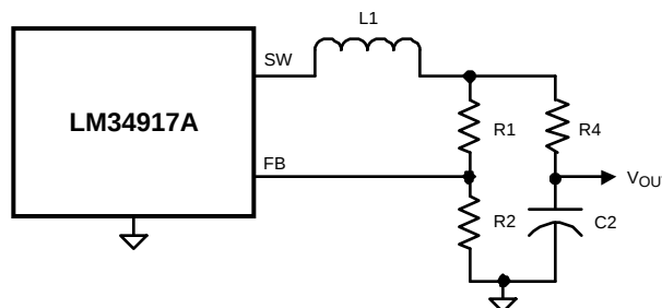
Figure 11. Alternate Minimum Output Ripple Configuration
