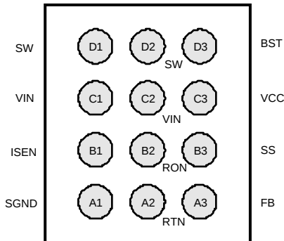
Figure 1. Bump Side
