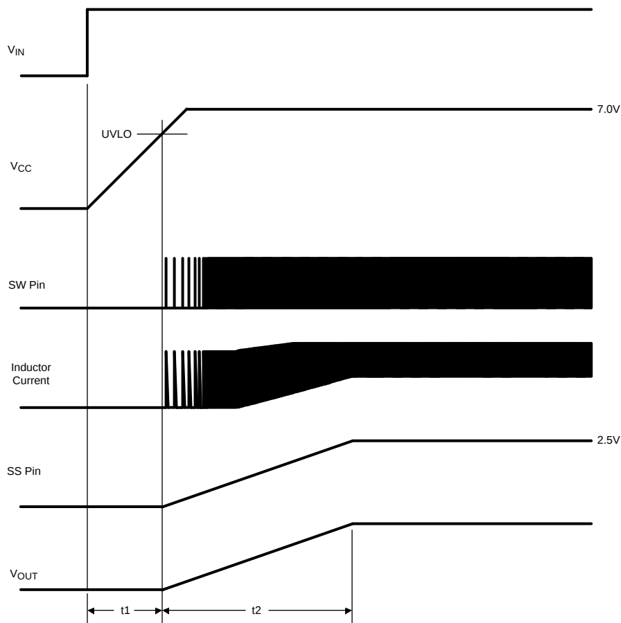
Figure 3. Startup Sequence
