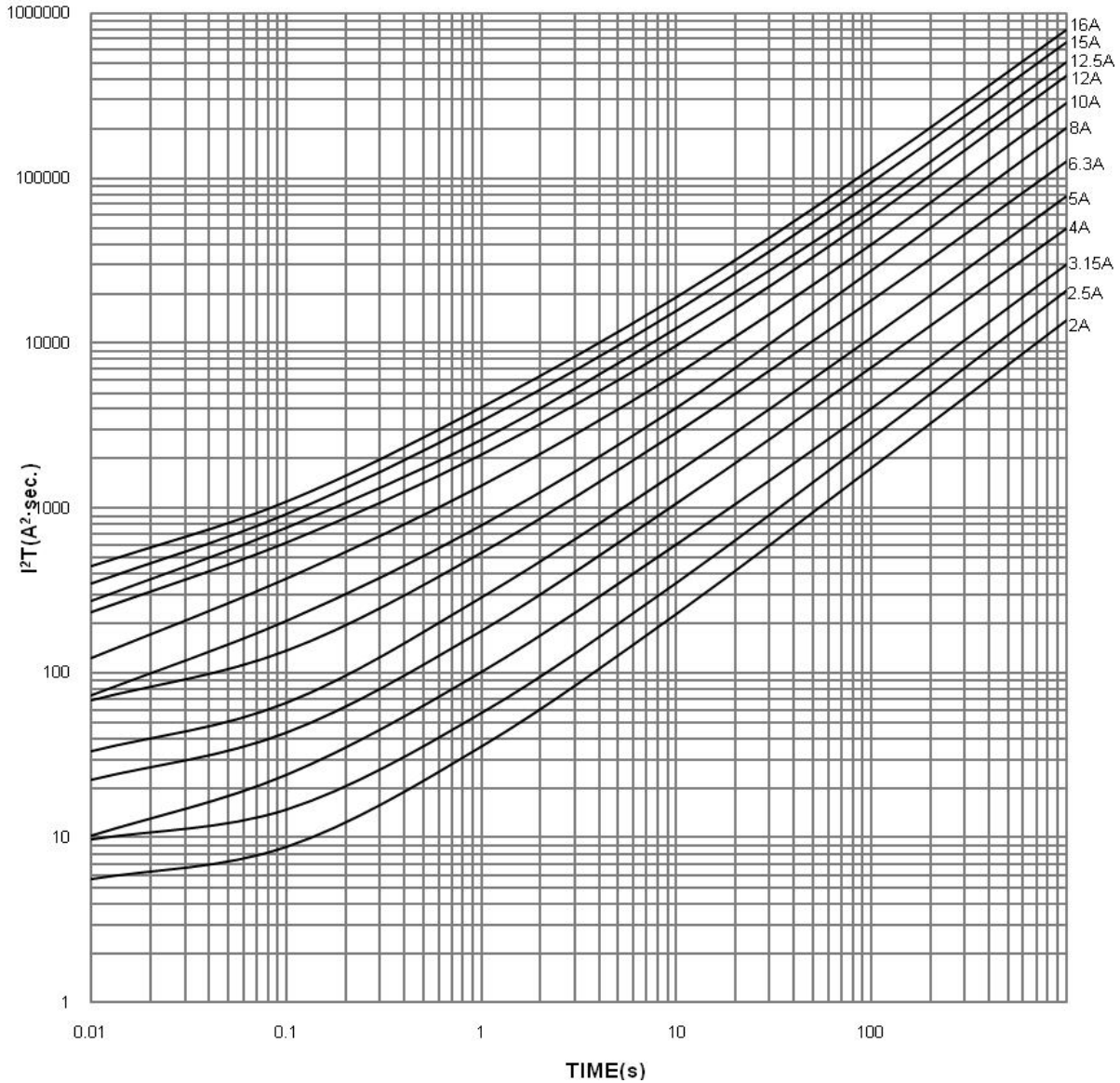
6.6 电压降、平均 I 2 T 值(供参考)、最大持续功耗/ VOLTAGE DROP, AVERAGE I 2 T VALUE(FOR REFERENCE ONLY) And MAXIMUM SUSTAINED DISSIPATION
