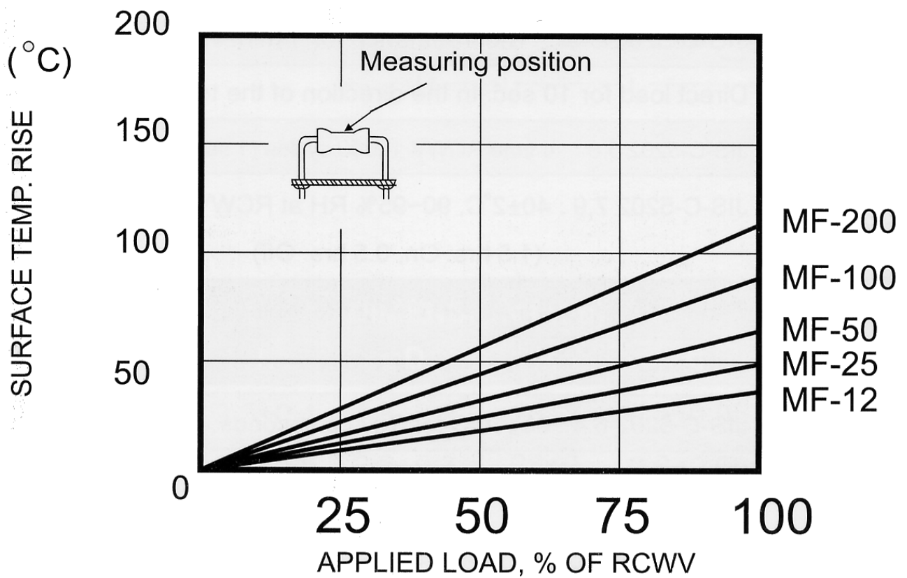
FIG.2 Hot-Spot Temperature
