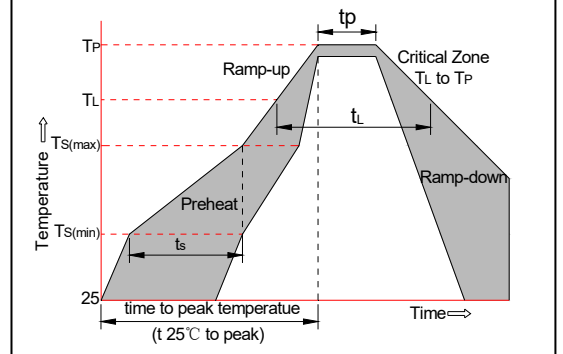
FIG.5: Reflow condition
