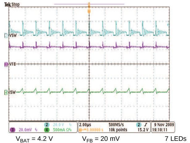
Figure 28. PWM Operation
