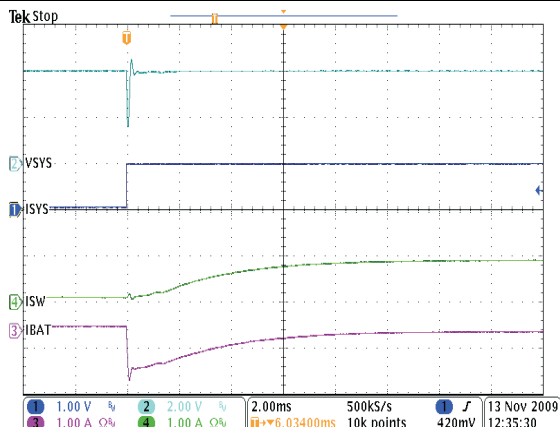
Figure 54. Transient Response
