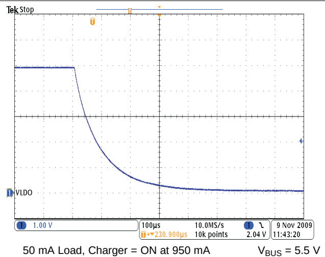
Figure 22. Shutdown
