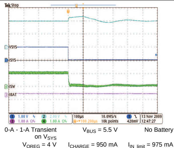
Figure 59. Transient Response
