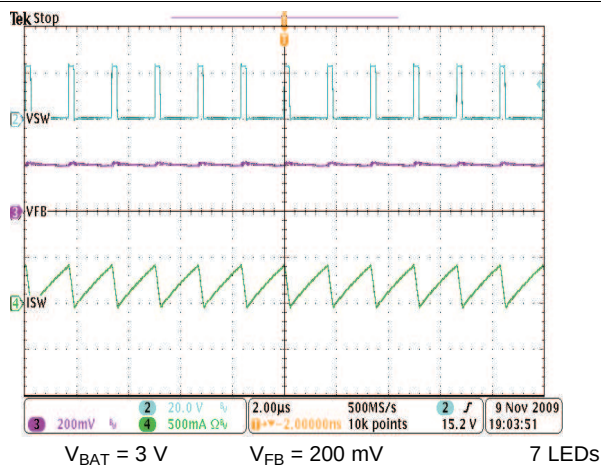
Figure 29. PWM Operation
