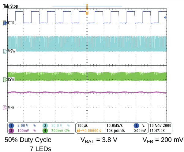
Figure 31. PWM Dimming
