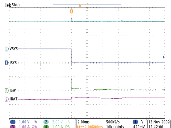
Figure 55. Transient Response
