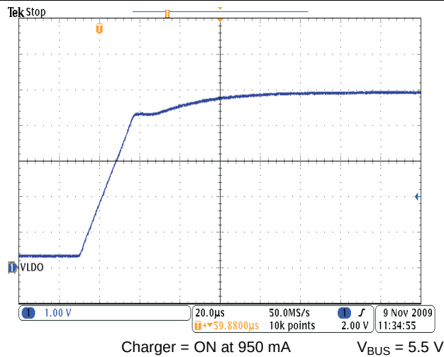
Figure 19. Start-Up
