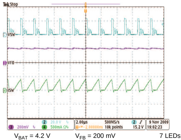
Figure 27. PWM Operation
