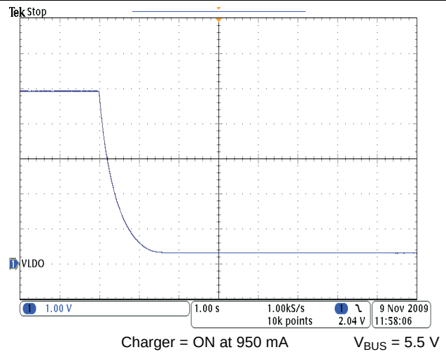
Figure 20. Shutdown
