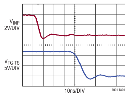
LTC7001 Driving a 1nF Capacitive Load
