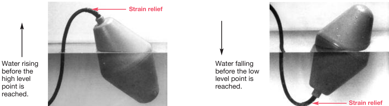
These photographs show the position of the float with rising and falling liquid level.
