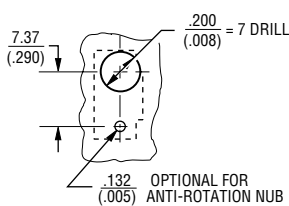
PANEL LAYOUT
