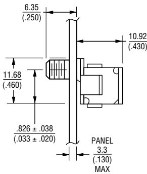
PANEL LAYOUT
