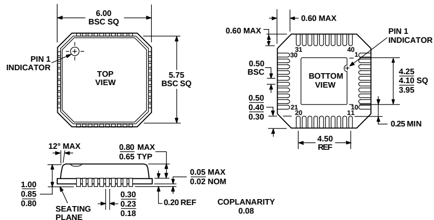
Figure 49. 40-Lead Lead Frame Chip Scale Package [LFCSP] (CP-40) Dimensions shown in millimeters
