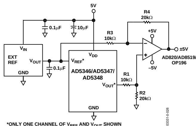
Figure 43. Bipolar Operation with the AD5346/AD5347/AD5348
