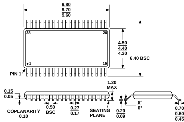
Figure 48. 38-Lead Thin Shrink Small Outline Package [TSSOP] (RU-38) Dimensions shown in millimeters
