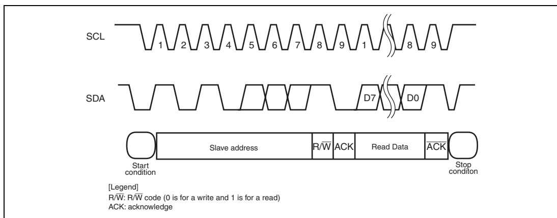
Figure 17.5 Current Address Read Operation
