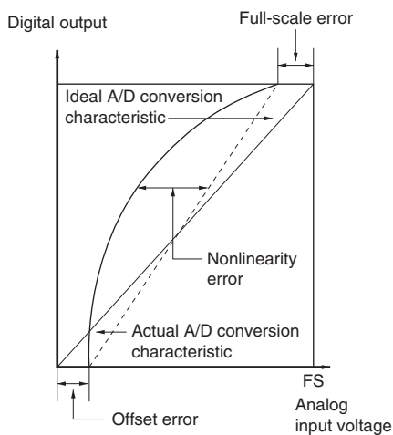
Figure 16.5 A/D Conversion Accuracy Definitions (2)
