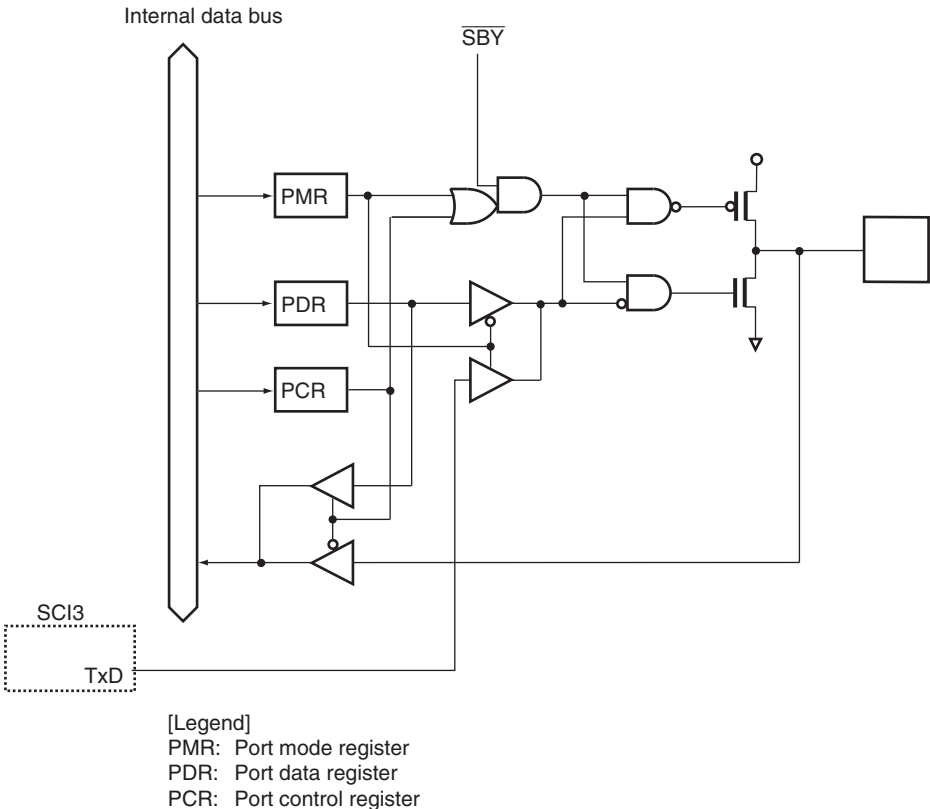
Figure B.5 Port 2 Block Diagram (P22)
